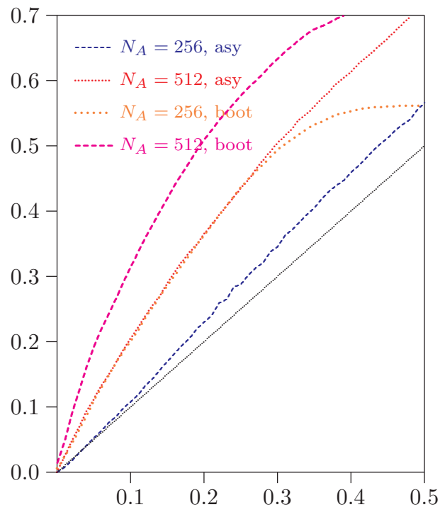
Figure 8: Power curves, z^- = 0.1 .
