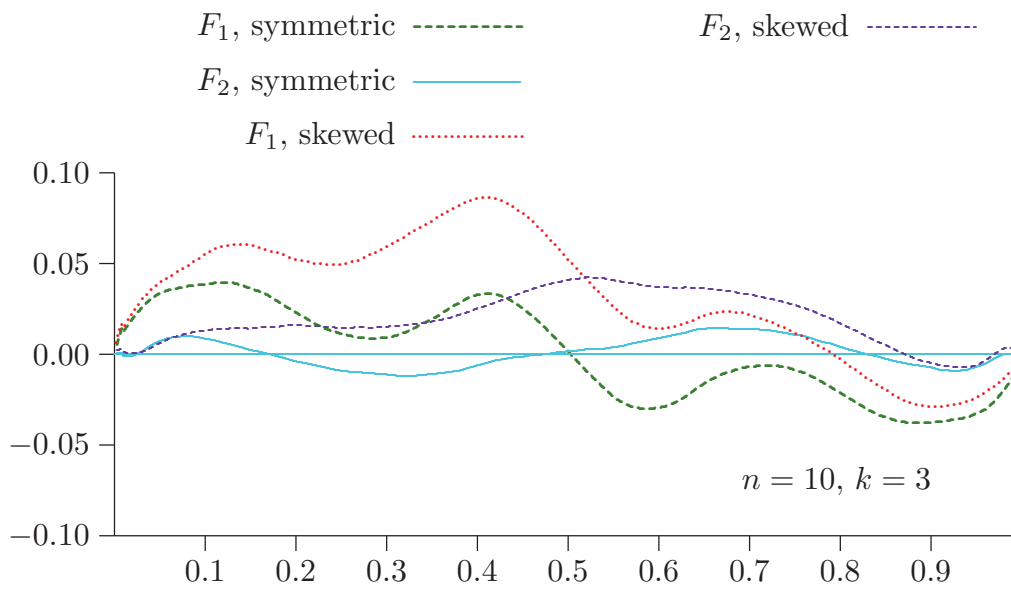
Figure 4. Homoskedastic errors
