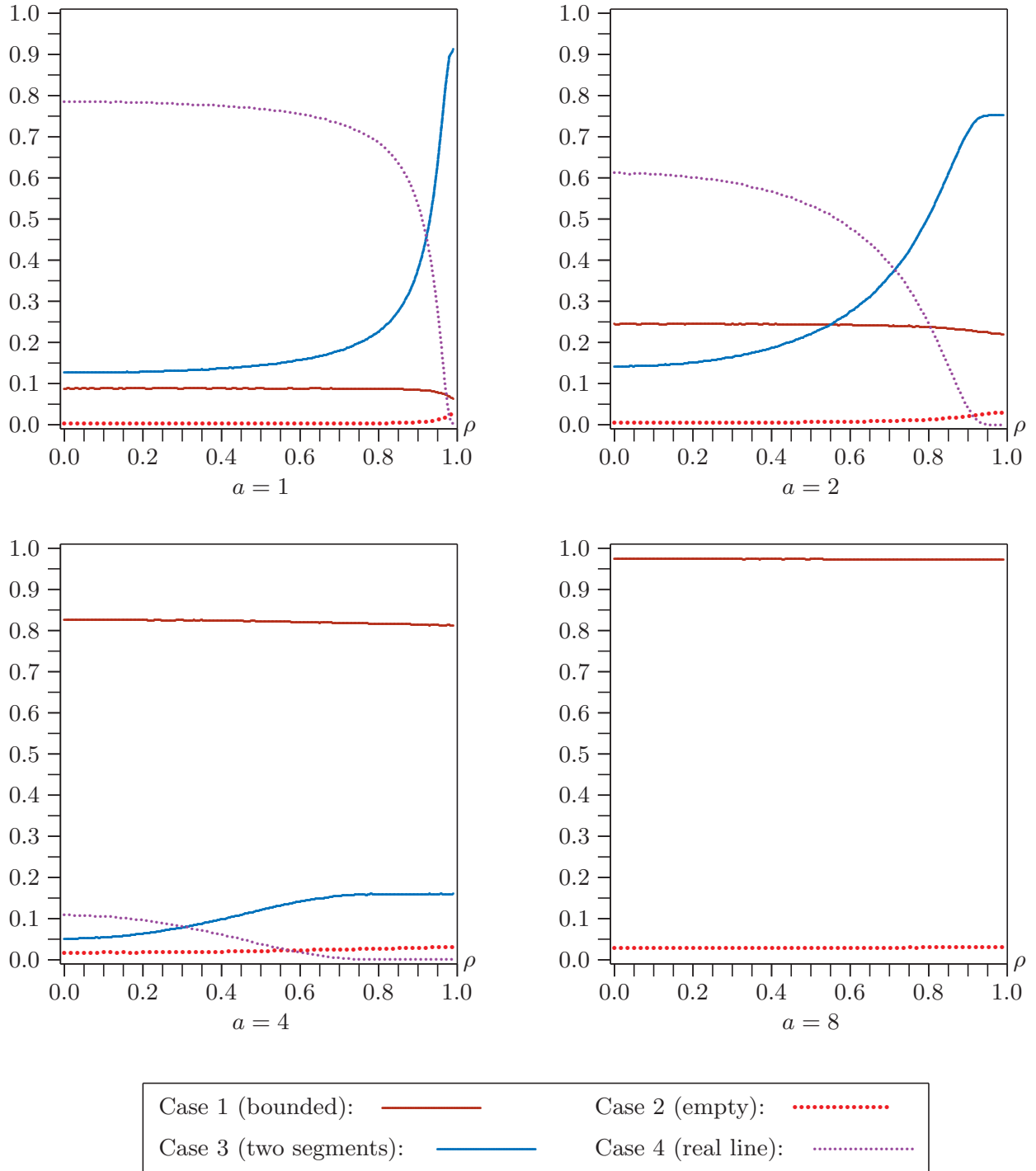
Figure 2. Frequencies of each type of confidence set as functions of \rho
