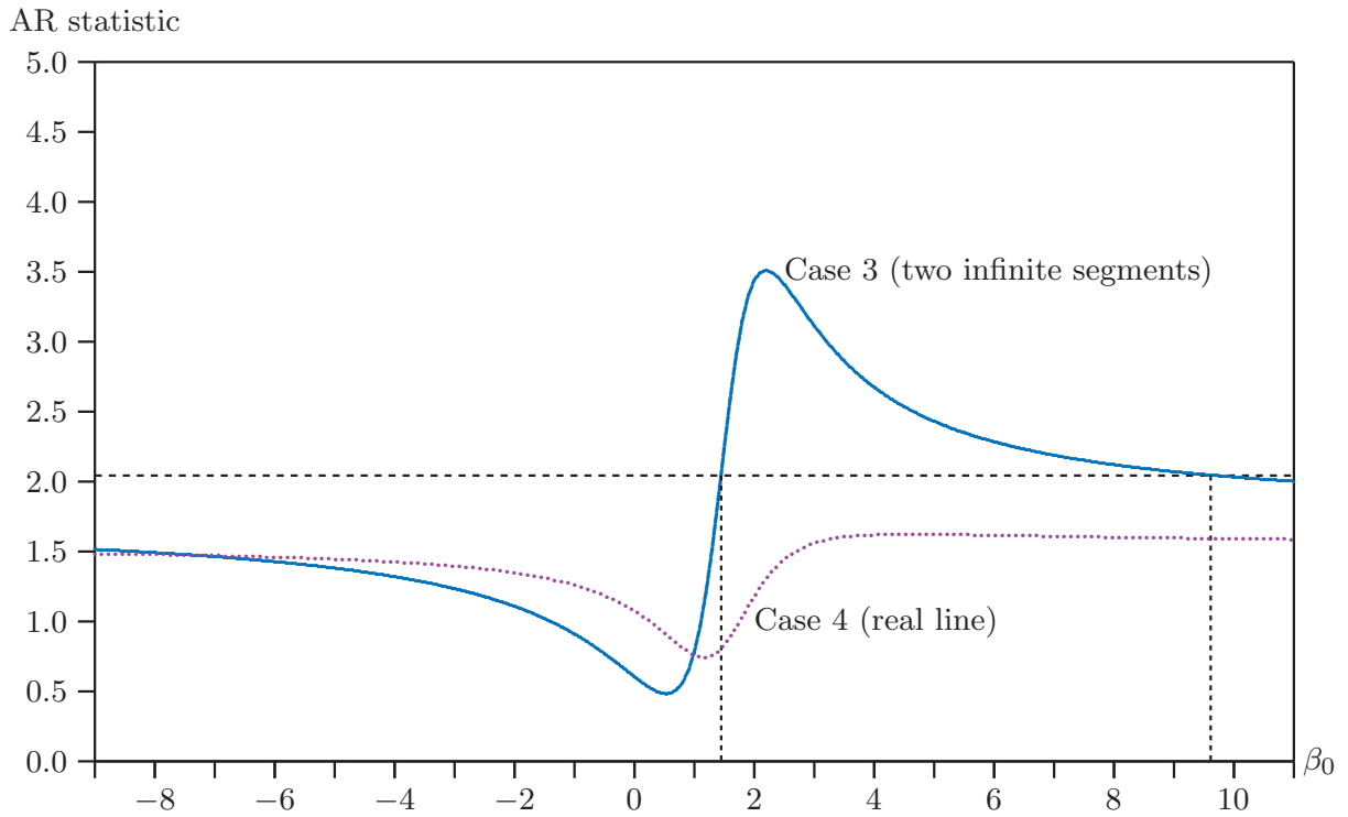
Figure 1. Five types of Anderson-Rubin confidence set
